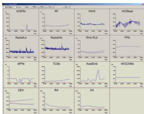
Defect Inspection
